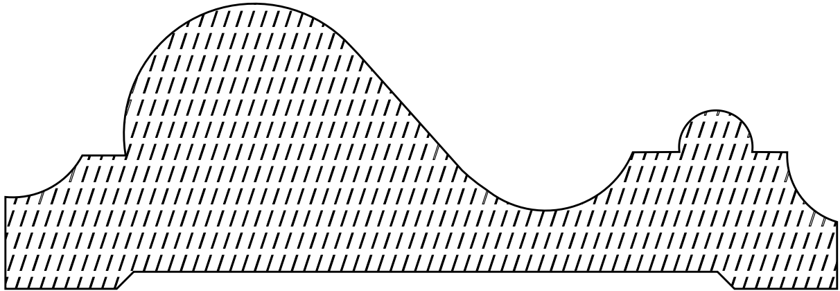
EM603BL 2.125" X 6.25"
