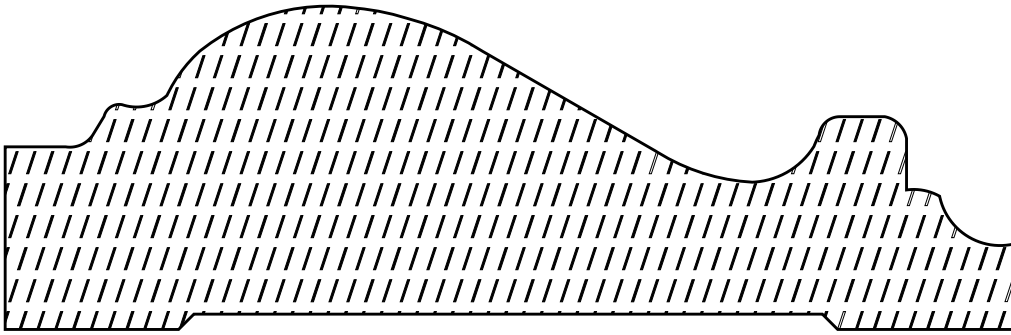
EM605BL 1.6875" X 5.25"
